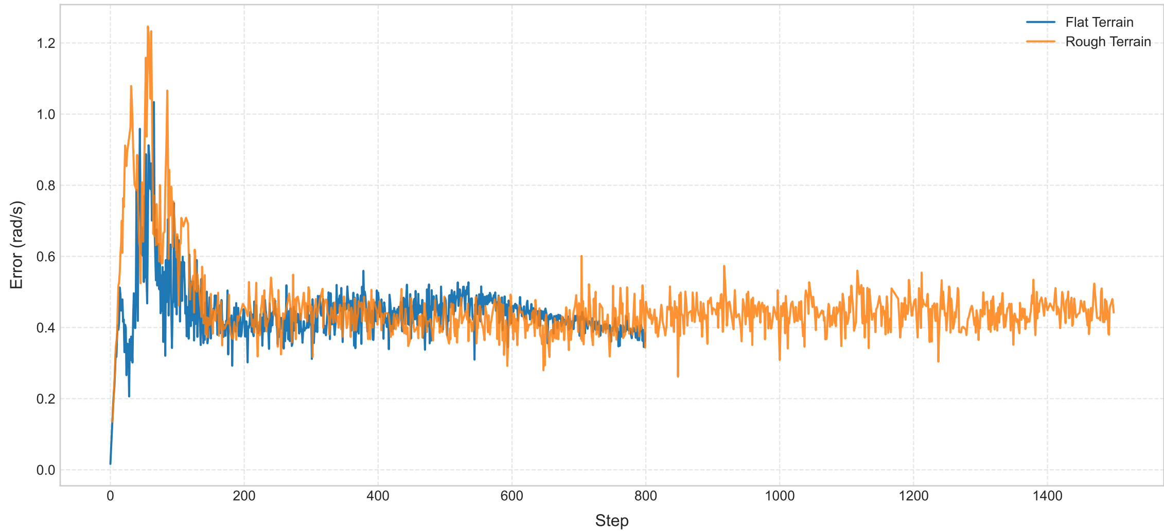
Yaw Velocity Tracking Error
